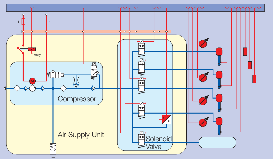
Four-corner air suspension with air reservoir and active shock absorber control (High Power Compressor)
