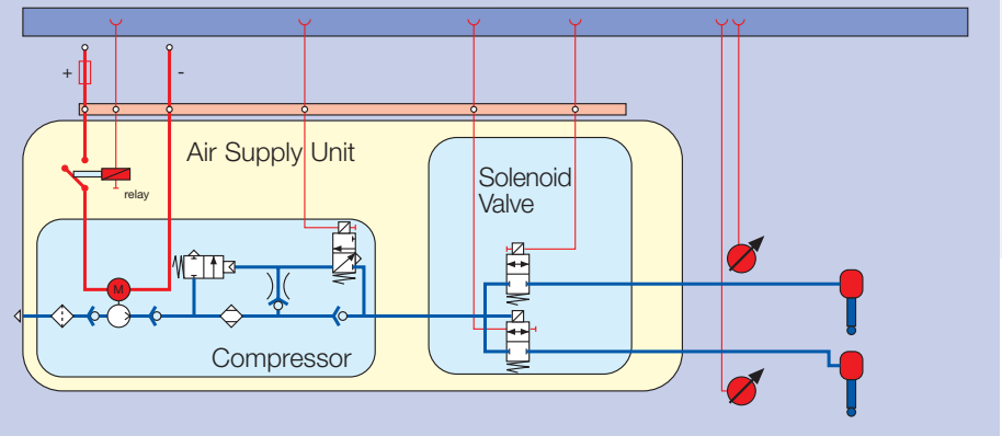
Rear axle air suspension (Medium Power Compressor)
